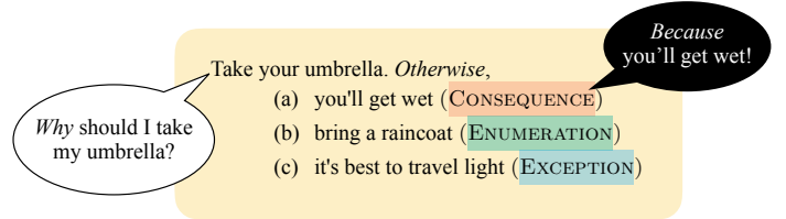
Figure 1: An example of otherwise functions.
