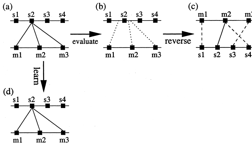
Figure 13 (a) Representation of an imitator agent's feed-forward network encoding an all-to-one p(m) mapping three meanings onto a single signal, s_2 . The function from a domain of real numbers (input unit activations) to a codomain of real numbers (output unit activations) is represented by two lines, the lower line representing the domain, the upper representing the codomain. Squares represent particular points on the line corresponding to binary meanings or signals. Associations are shown with solid lines between elements in the domain and elements in the codomain. (b) The confidence-measuring step of the reversal process for the network underlying (a). To decide r(s_2) , the real-number values of p(m_1) , p(m_2) and p(m_3) are calculated. These real-numbered mappings are represented by dotted lines in (b). (c) The r(s) derived from applying the reversal process to (a). r(s_2) = m_2 because m_2 mapped closer to s_2 than any other m in (b). The other associations are effectively random. The random nature of these mappings is represented by dashed lines. (d) The function acquired by an imitator network exposed to behavior generated by (a)—as it is an all-to-one function between meanings and signals it is easily learned by imitator agents. This is in fact the only stable function for imitators.
