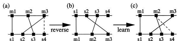
Figure 15 Only an unambiguous p(m) is stable for obverter agents. (a) An obverter agent's r(s) . (b) The p(m) derived from reversal of (a)—it is an injective function. (c) The r(s) resulting from training the next generation of agents on data produced by (b) is effectively similar to (a) and will therefore lead to (b) once again—(a) and (b) are culturally stable. The only unstable aspect is the floating synonym s4 . This synonym is highly unlikely to interfere with the mapping in (b) and the floating synonym phenomenon can be observed in the other obverter models outlined in the main text.
